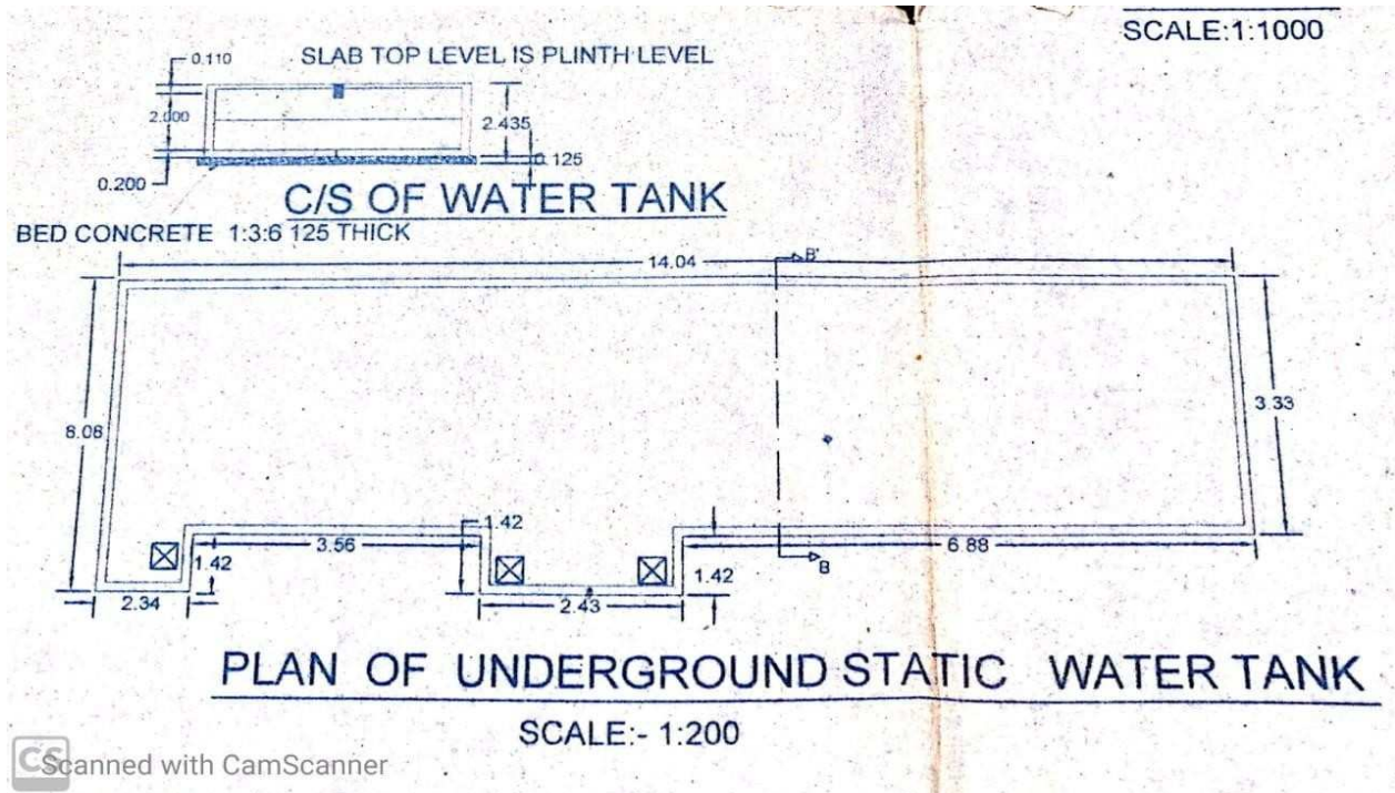
Map of the Tank of Rain water Harvesting at college campus – Girls Hostel Building
