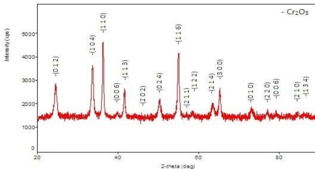
Fig. 1: X-ray diffraction pattern of \text{Cr}_2\text{O}_3 powder sample calcinated at 600^\circ\text{C} .
