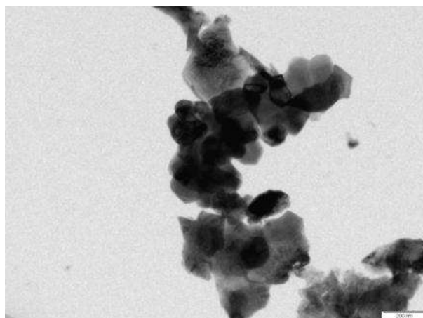
Figure 3(a). TEM image of nanocrystalline Mg_{0.5}Zn_{0.5}Fe_2O_4 .
