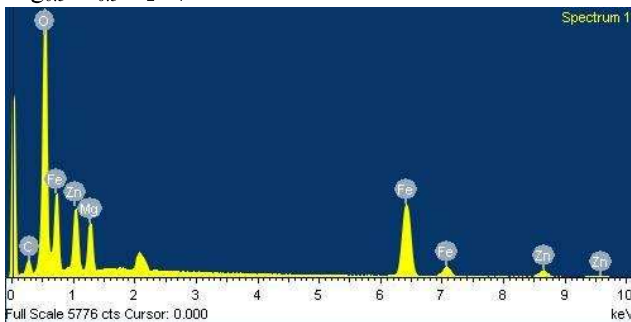
Figure 5. EDX spectrum for nanocrystalline Mg_{0.5}Zn_{0.5}Fe_2O_4 .
