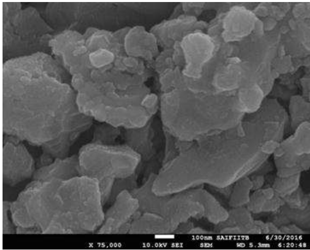
Figure 4. SEM image of nanocrystalline Mg_{0.5}Zn_{0.5}Fe_2O_4 .
