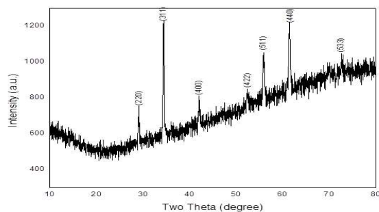
Figure 1. XRD pattern of Mg_{0.5}Zn_{0.5}Fe_2O_4 calcinated at 700^\circ C .
