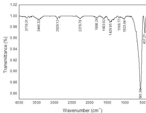
Figure 2. FTIR spectrum of nanocrystalline Mg_{0.5}Zn_{0.5}Fe_2O_4 .
