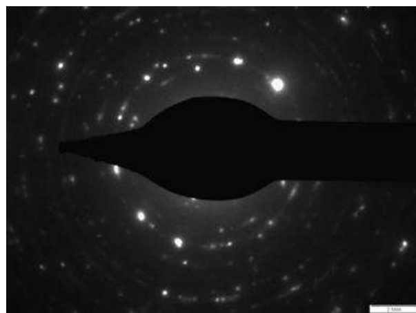
Figure 3(b). SAED micrograph of nanocrystalline Mg_{0.5}Zn_{0.5}Fe_2O_4 .
