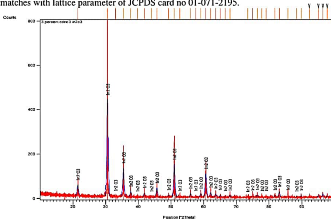
Fig. 1: X-ray diffraction pattern pattern of 3wt% Cd doped In 2 O 3 powder.
