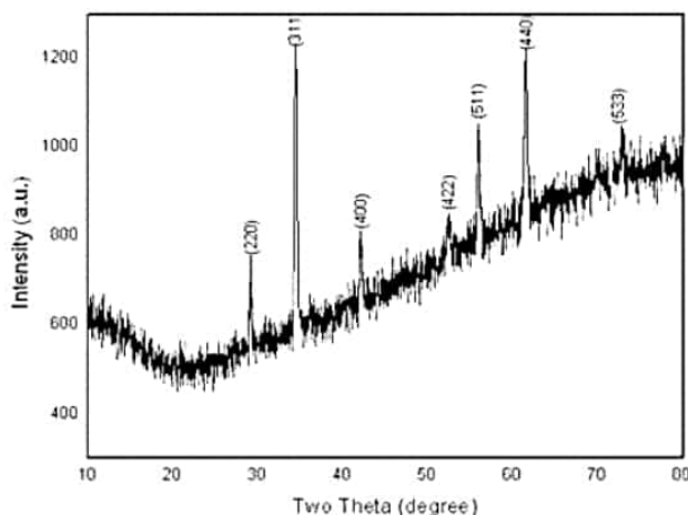
Fig. 1. XRD pattern of Mg_{0.5}Zn_{0.5}Fe_2O_4 calcined at 700^\circ C .
