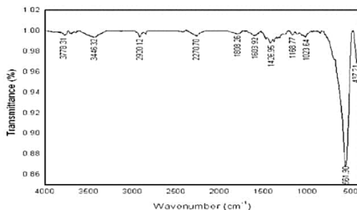
Fig. 2. FTIR spectrum of nanocrystalline Mg_{0.5}Zn_{0.5}Fe_2O_4 .
