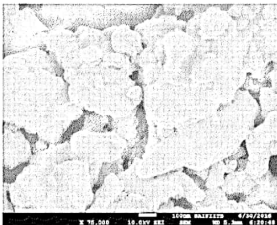
Fig. 4. SEM image of nanocrystalline Mg_{0.5}Zn_{0.5}Fe_2O_4 .
