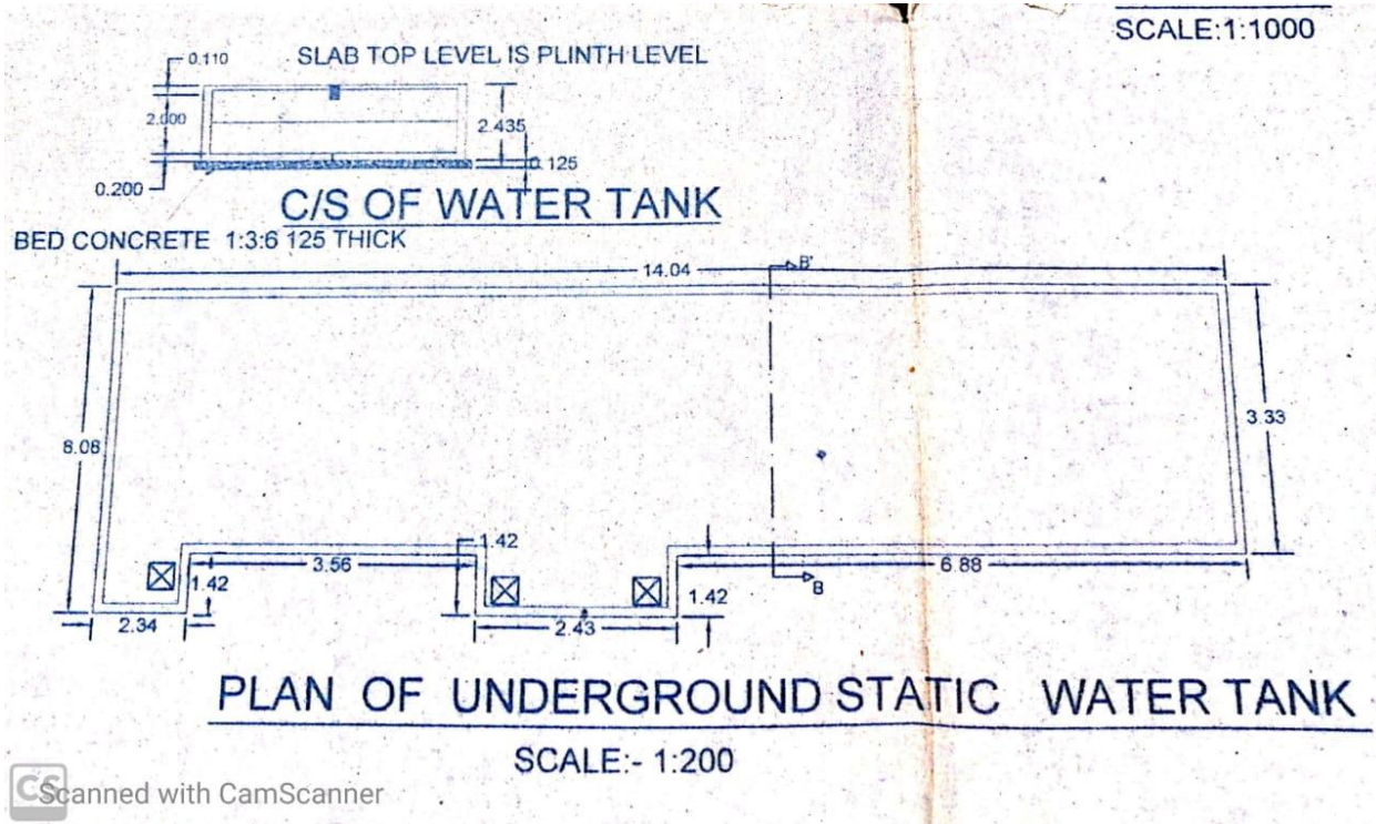
Map of the Tank of Rain water Harwaisting at college campus - Girls Hostel Building
